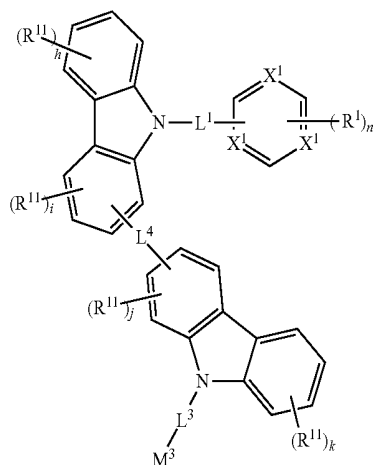
[Formula 6]
