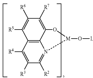
[Formula 239]
