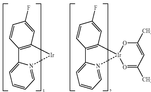
[Formula 232]
