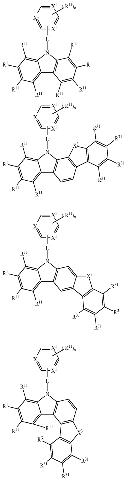
[Formula 9]
