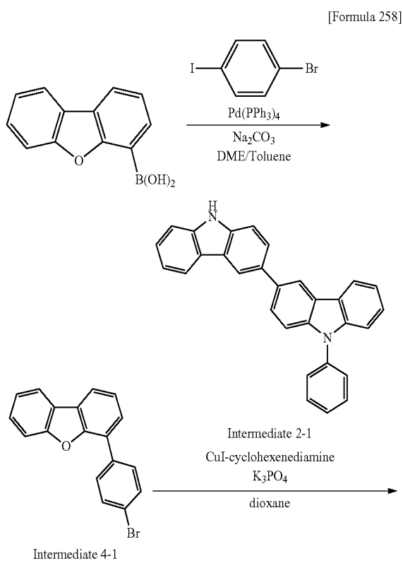
Intermediate 4-1
