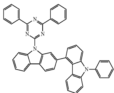
[Formula 72]
