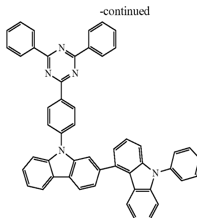
[Formula 73]
