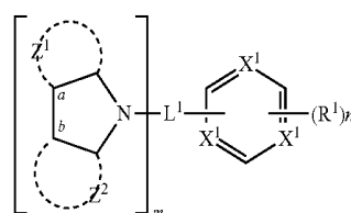
[Formula 4]
