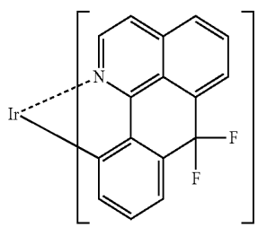
[Formula 232]
