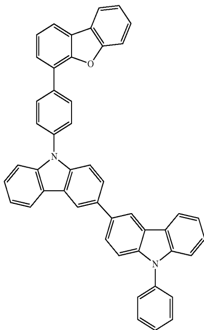
Compound GH2-3
