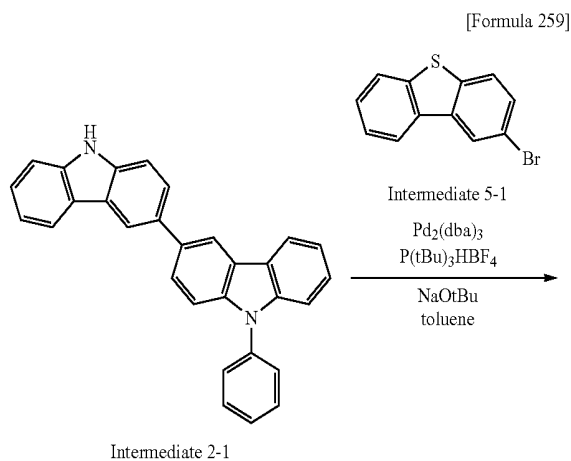
Intermediate 2-1
