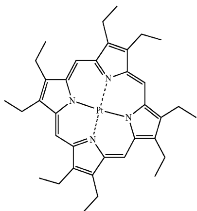
[Formula 231]
