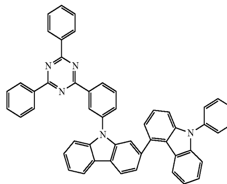
[Formula 73]
