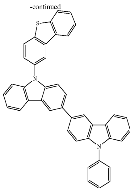
Compound GH2-4
