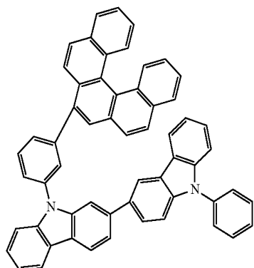
[Formula 117]
