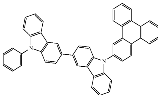
[Formula 261]
