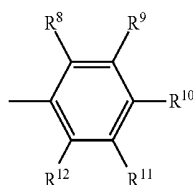
[Formula 240]
