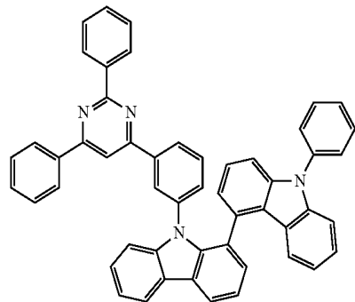
[Formula 72]
