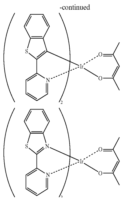
[Formula 231]
