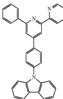
[Formula 10]
