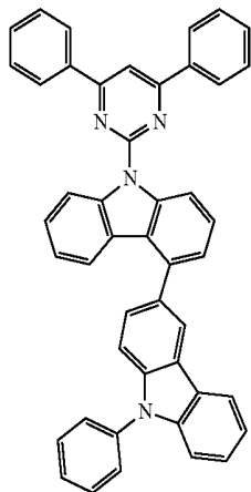
[Formula 57]
