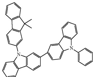
[Formula 117]
