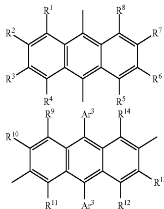
[Formula 249]
