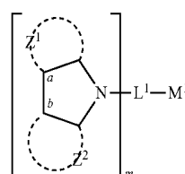
[Formula 1]
