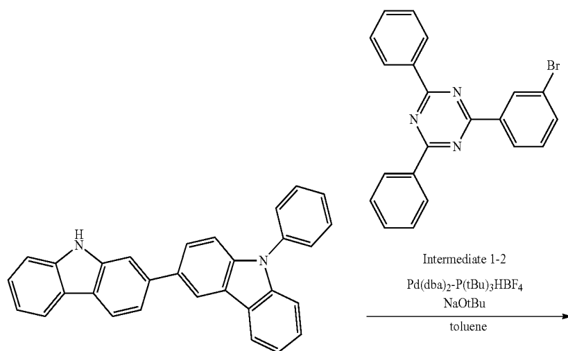
Intermediate 1-3
