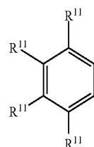
[Formula 2]
